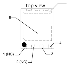
Package Outline
