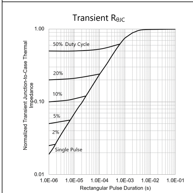
Figure 15: Transient Thermal Impedance (1.00 = Nominal DC thermal impedance)
