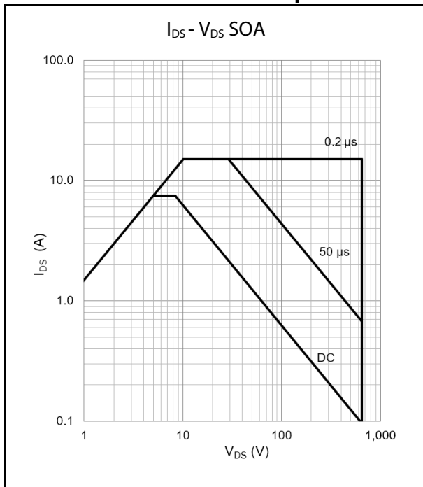
Figure 13: Safe Operating Area @ T_{case} = 25\text{ °C}
