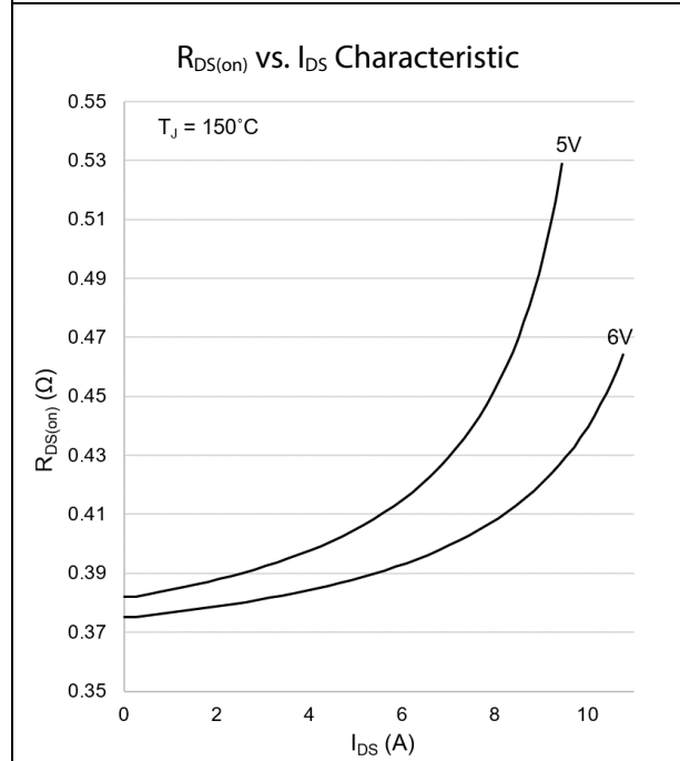
Figure 4: R_{DS(on)} vs. I_{DS} at T_J = 150\text{ }^\circ\text{C}
