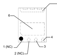
Package Outline
