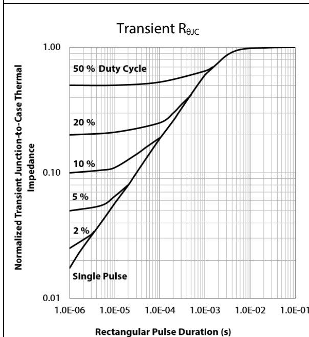
Figure 14: Transient Thermal Impedance 1.00 = Nominal DC thermal impedance
