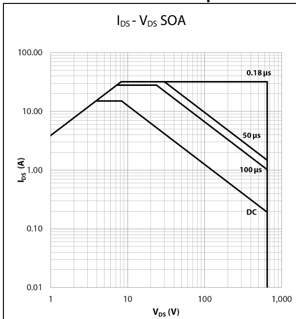
Figure 12: Safe Operating Area @ T case = 25 °C
