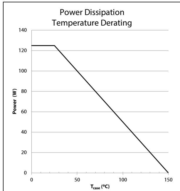
Figure 13: Power Derating vs. T case
