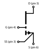
Circuit Symbol
