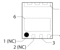
Package Outline
