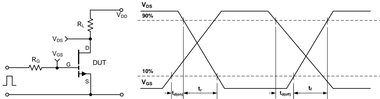
Figure 15: GS66516T switching time test circuit and waveforms
