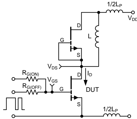
Figure 16: GS66516T Switching Loss Test Circuit
