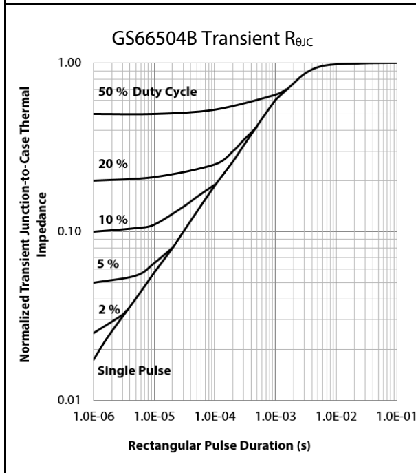
Figure 16: Transient Thermal Impedance
