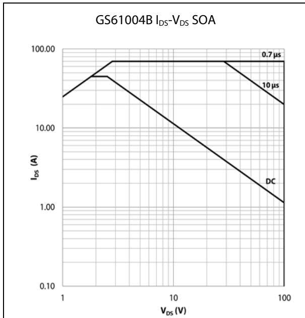
Figure 14: Safe Operating Area @ T_{case} = 25\text{ }^{\circ}\text{C}
