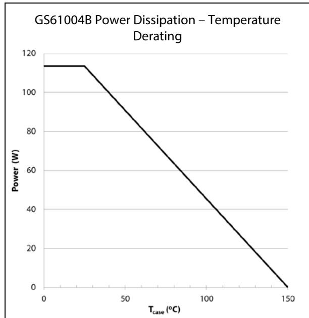
Figure 15: Derating vs. Case Temperature
